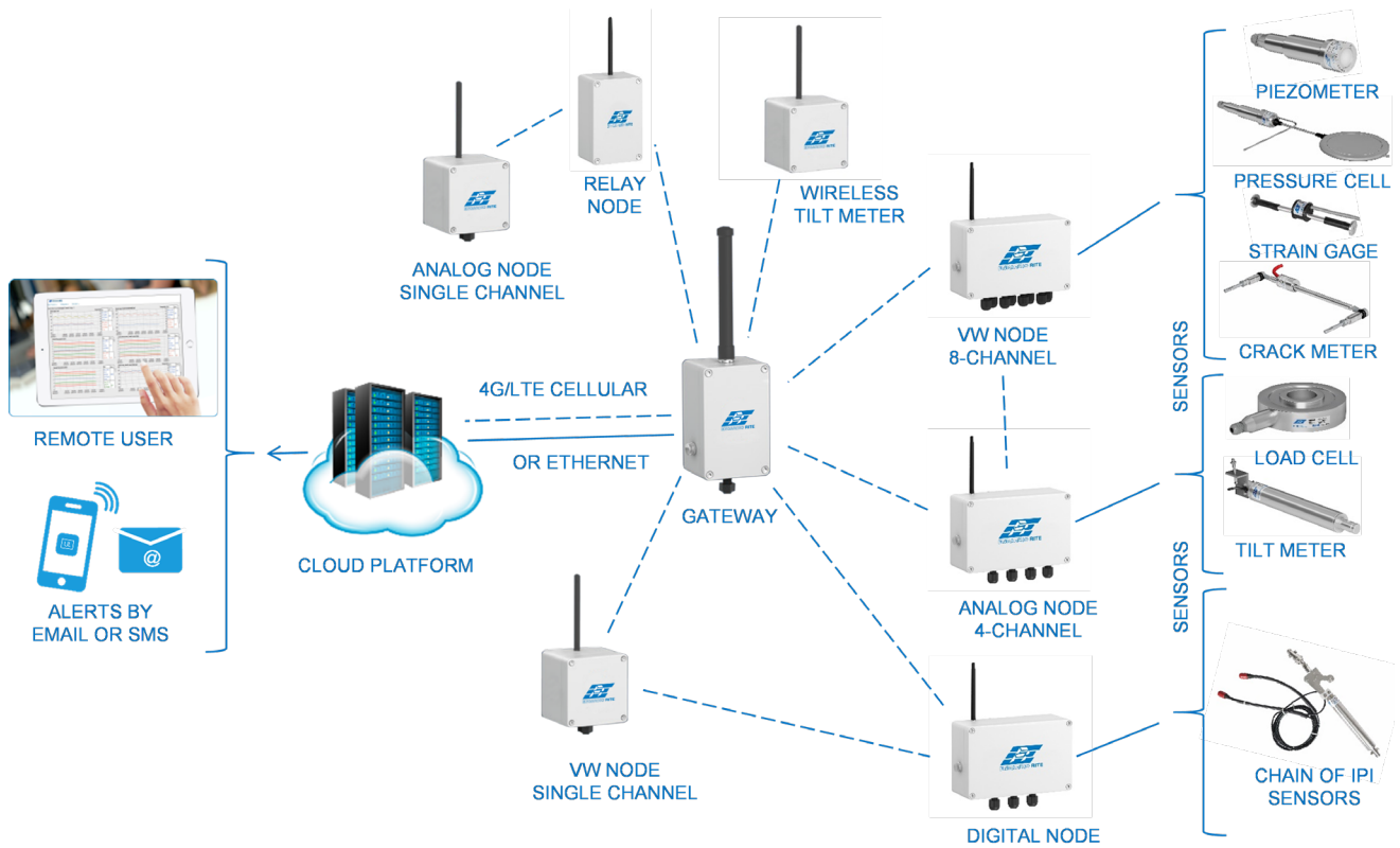
Remote real-time monitoring system with wireless (RF) nodes and gateways
