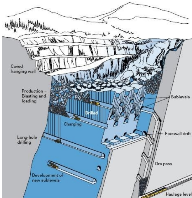
Block caving mining
